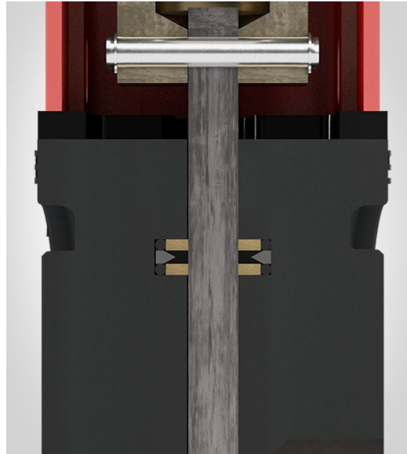
Unique transverse seal
